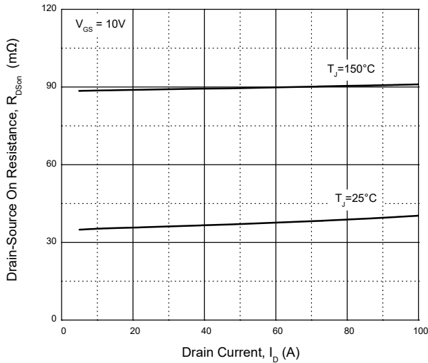
Fig. 3 - Drain-Source On-Resistance
