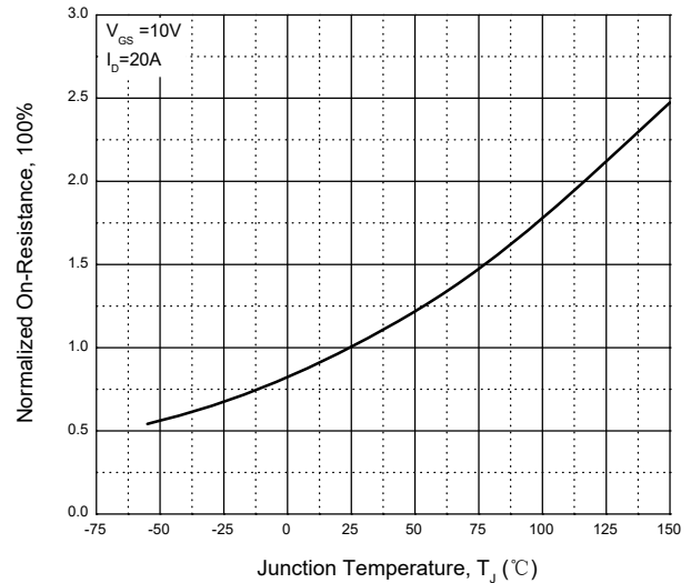
Fig. 4 - Normalized On-Resistance
