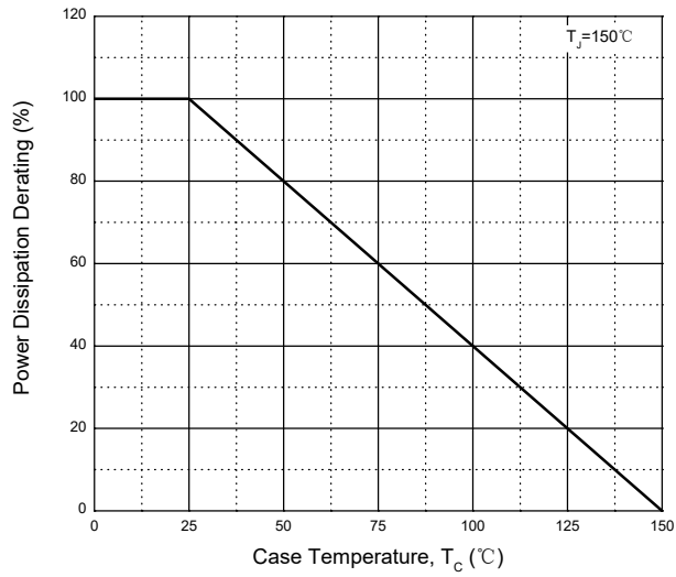
Fig. 12 - Power Derating
