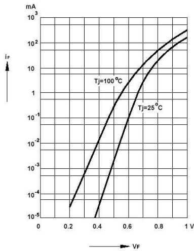
Forward characteristics
