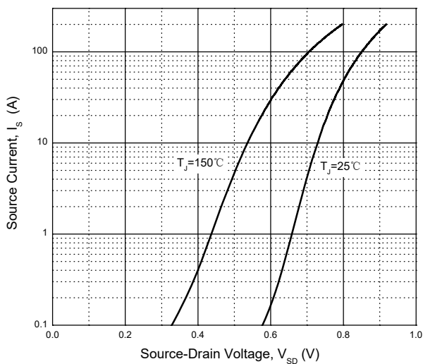
Fig. 9 - Forward Characteristic
