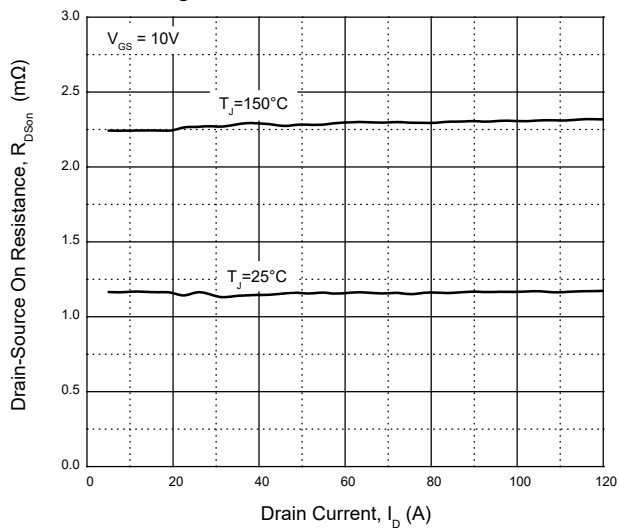
Fig. 3 - Drain-Source On-Resistance
