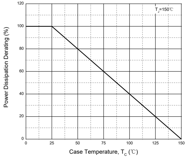
Fig. 12 - Power Derating
