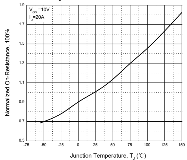
Fig. 4 - Normalized On-Resistance
