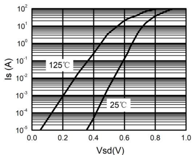
Fig.6 - Forward Characteristic
