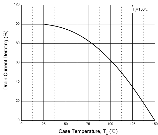
Fig. 12 - Drain Current Derating
