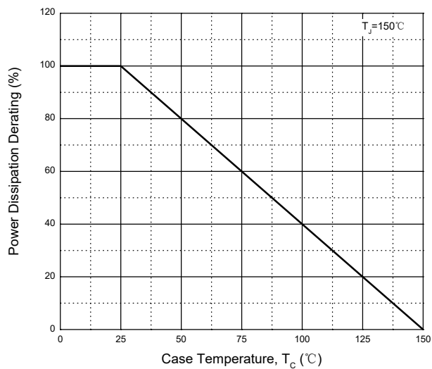
Fig. 11 - Power Derating
