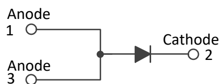
TO-252 (D-PAK)
