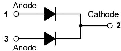
TO-220AB
